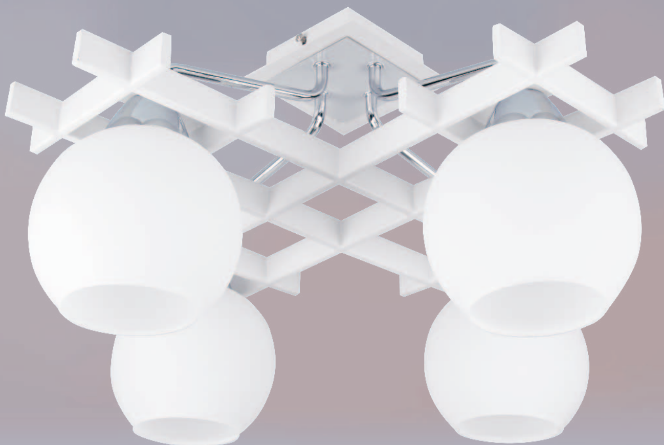
Leonie 002 ↑ 26, ↔ 51 4xE14x40W
